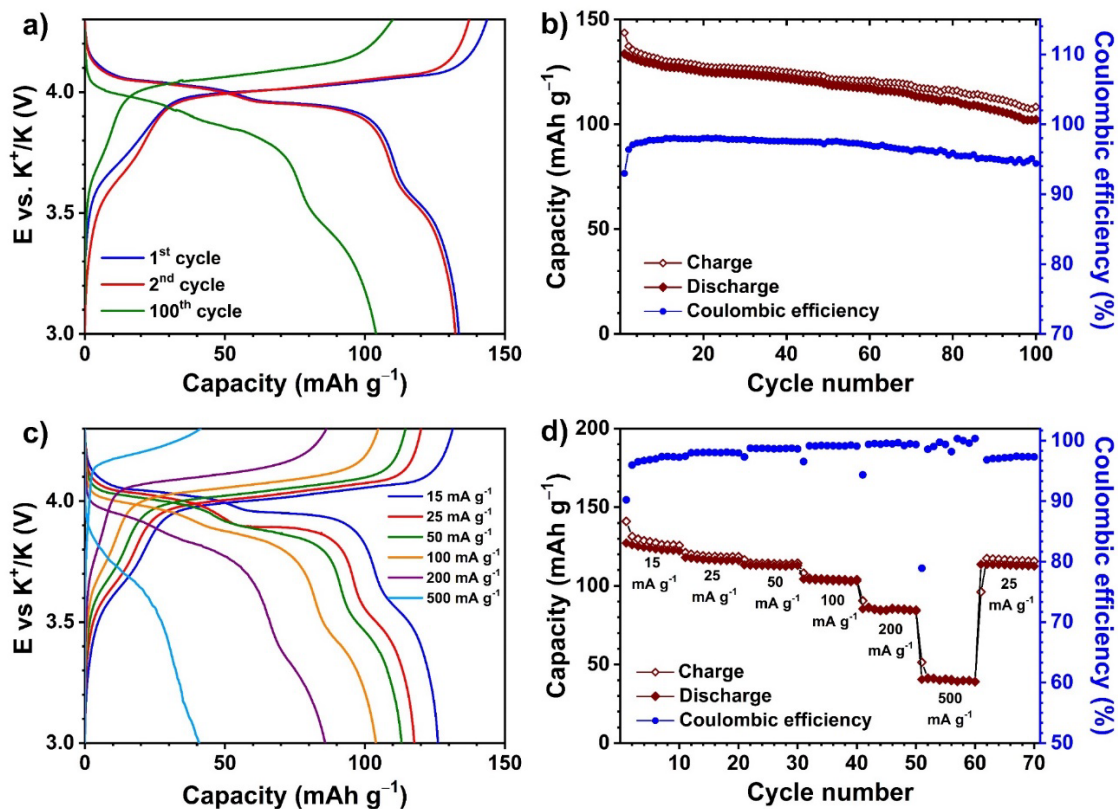
Figure 2. (a, b) Galvanostatic profile and cyclability of MF21 at a constant current of 25 mA g -1 , respectively; (c) cycling profiles and (d) rate capability of MF21 at currents varying between 15 and 500 mA g -1 .
