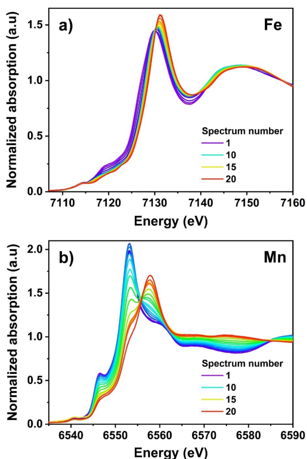
Figure 7. Operando XANES at the Fe (a) and Mn (b) K edges in the MF21|K PIB in situ half-cells during the first charge (depotassiation).
