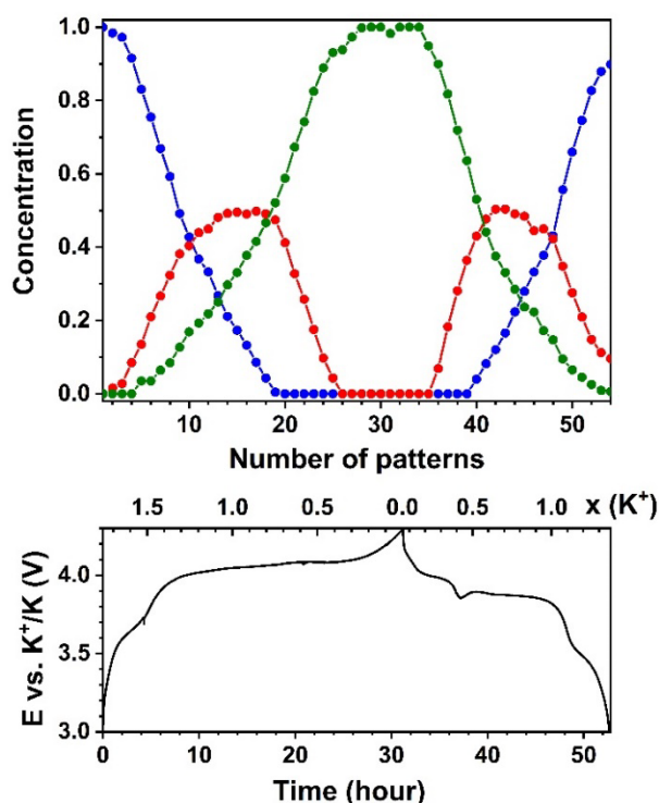
Figure 5. Evolution of the relative contributions of the three pure components (Component 1: blue, Component 2: red, Component 3: green) obtained from the PCA and MCR-ALS treatment of the operando XRD in the first cycle (top) and the corresponded cycling profile at 5 mA g^{-1} (bottom).
