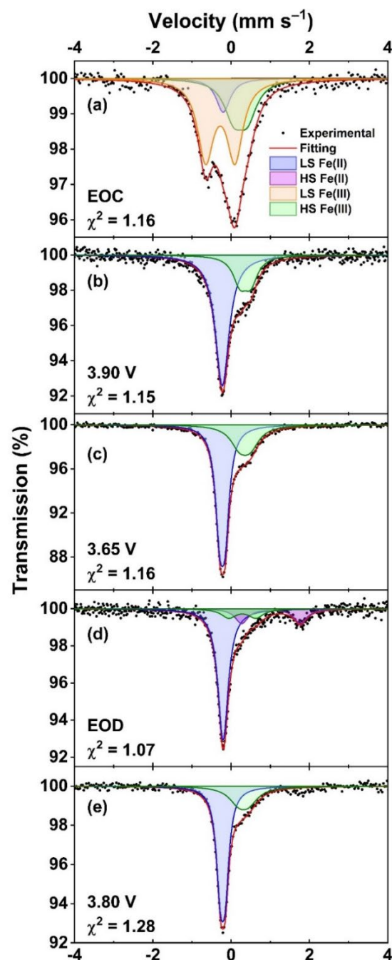
Figure 3. Room temperature ex situ Mössbauer spectra of MF21 recorded at different states: (a) 4.3 V – end of charge (EOC), (b) 3.90 V (end of plateau 1 in the discharge), (c) 3.65 V (end of plateau 2 in the discharge), (d) 3.0 V – end of discharge (EOD), and (e) 3.80 V (end of plateau 3 in the charge).
