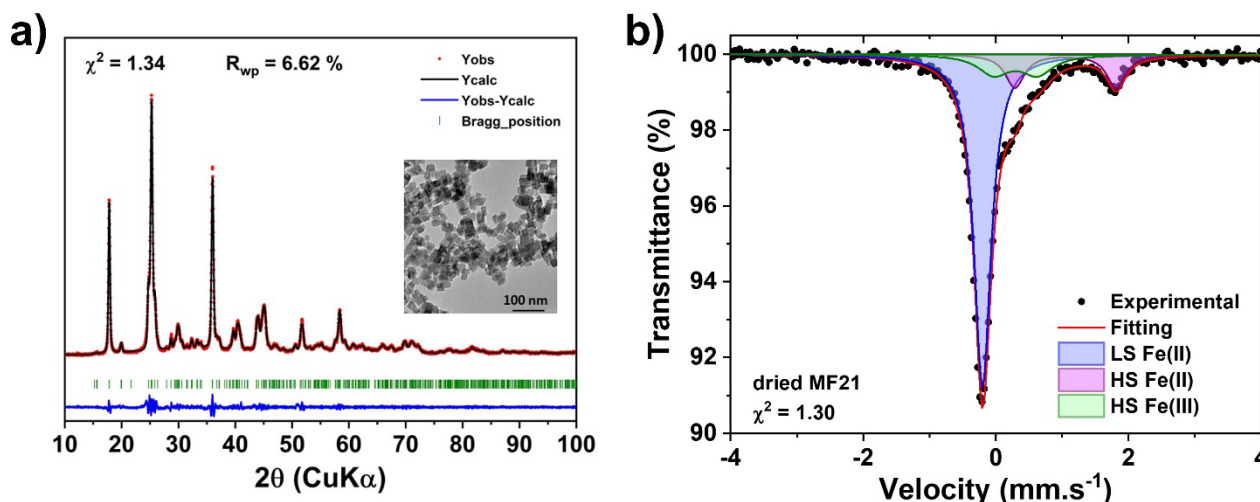
Figure 1. (a) XRD pattern of MF21 dried at 100°C with Rietveld refinement and TEM image (inset) and (b) Mössbauer spectrum of dried MF21
