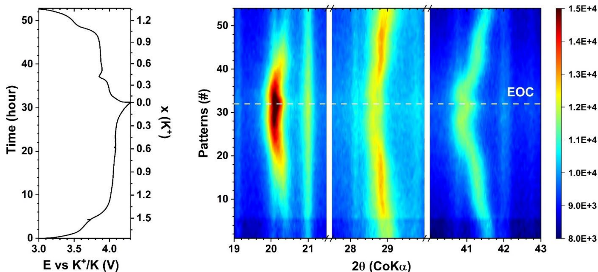
Figure 4. Operando XRD contour map for three selected 2\theta regions of MF21 recorded at the current density of 5 mA/g, in the voltage range of 3 – 4.3 V (vs. K + /K) using the 5 M KTFSl in DME electrolyte.
