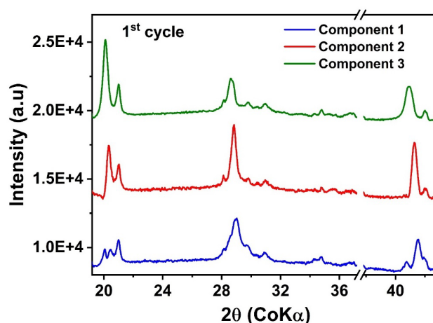
Figure 6. Computed XRD patterns of the three MCR-ALS components.
