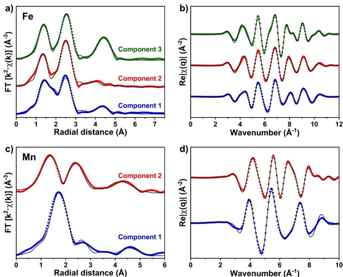
Figure 11. Fit of the modulus of the k^2 -weighted \chi(R) of the Fe (a) and Mn (c) K-edge MCR-ALS pure components performed in the R -range 1.0 – 5.5 Å. The \chi(R) were extracted from the corresponding EXAFS signals using the k -ranges 3 – 11.5 Å -1 and 3 – 9.855 Å -1 for the Fe and Mn K-edge, respectively, using a sine window. (b) and (d) are the corresponding fits of the real part of \chi(q) corresponding to the backward FT of \chi(R) in the R -range of 1.0 – 5.5 Å. The circles represent the experimental data, and the solid lines represent the fits.
