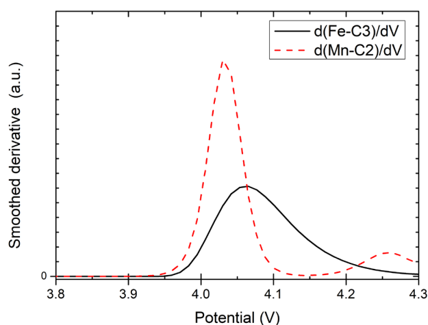
Figure 10. Smoothed derivatives of the concentration of the MCR-ALS pure Component 3 of the Fe K-edge dataset and of Component 2 of the Mn K-edge dataset (cf. Figure 9).
