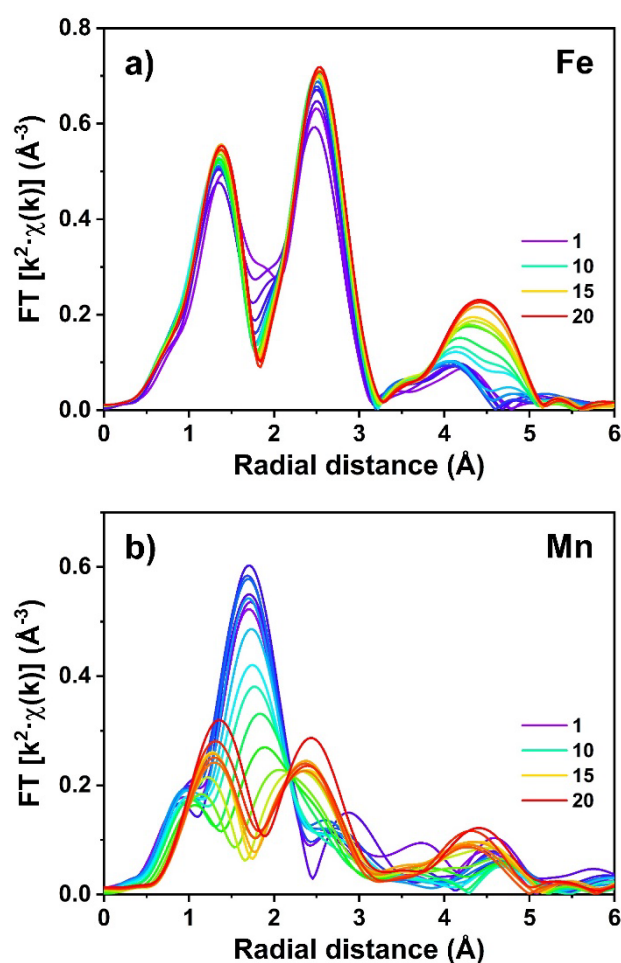
Figure 8. Evolution of the FT of the EXAFS of Fe (a) and Mn (b) during the first charge (depotassiation) of MF21.
