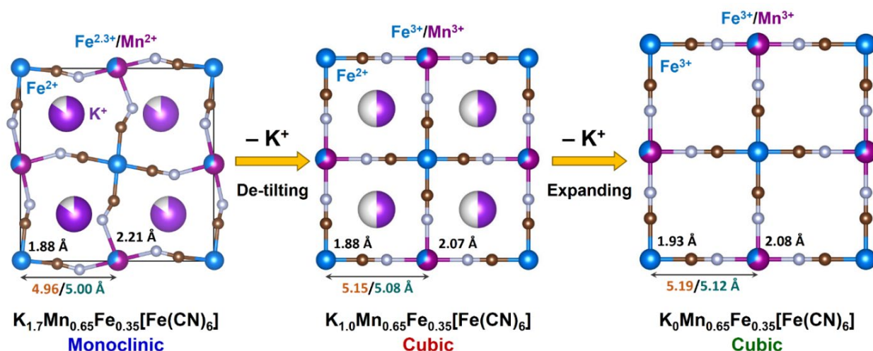
Figure 12. Schematic phase transition occurring in the depotassiation by combining operando XRD and XAS analysis. The M–N (M= Fe, Mn) bond lengths are the mean values calculated from EXAFS fits of pure components. The Fe–C–N–M distances are deduced from mean values of EXAFS fit data (orange) and lattice parameters of XRD pure components (dark teal).
