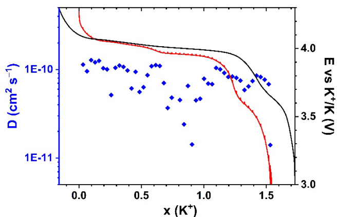
Figure 13. Evolution of diffusion coefficients of K^+ in the first discharge (blue diamonds) with the first charge (black line) and GITT curve (red line) of the discharge.
