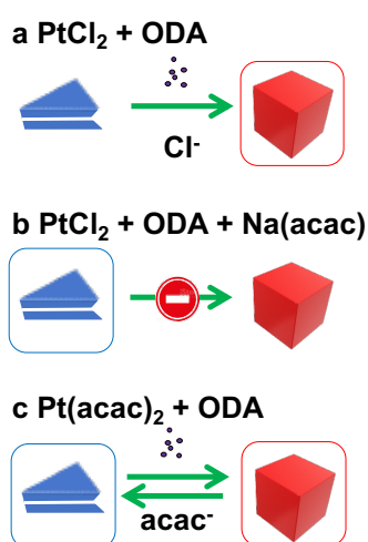
Scheme 1. Qualitative representation of the nucleation pathways for each case discussed. The framed nano-objects correspond to the structures that survive after the nucleation step. Twinned seeds are represented as blue triangles and defect-free seeds as red cubes. (a) \text{PtCl}_2 in the presence of ODA. The \text{Cl}^- ions liberated remain in the reaction medium and
