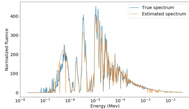
Fig. 3. Example of an estimated spectrum using our model. The normalized fluence corresponds to the fluence divided by the energy interval and the x-axis is “log” scaled.
