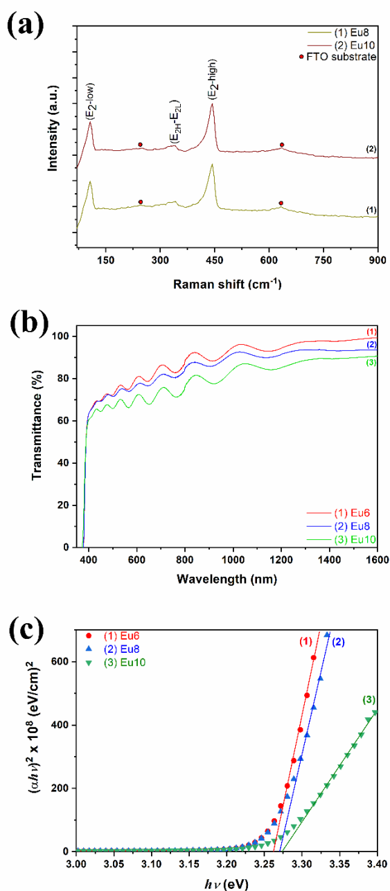
Figure 5. (a) Raman spectra of ZnO:Eu nanowires deposited with different Eu content: (1) 8 μM; and (2) 10 μM. (b) Transmission spectra of ZnO:Eu nanowires with different Eu content: (1) 6 μM; (2) 8 μM; and (3) 10 μM. (c) Plot of (αhν) 2 vs (hν) for ZnO:Eu nanowires with different Eu content: (1) 6 μM; (2) 8 μM and (3) 10 μM.
