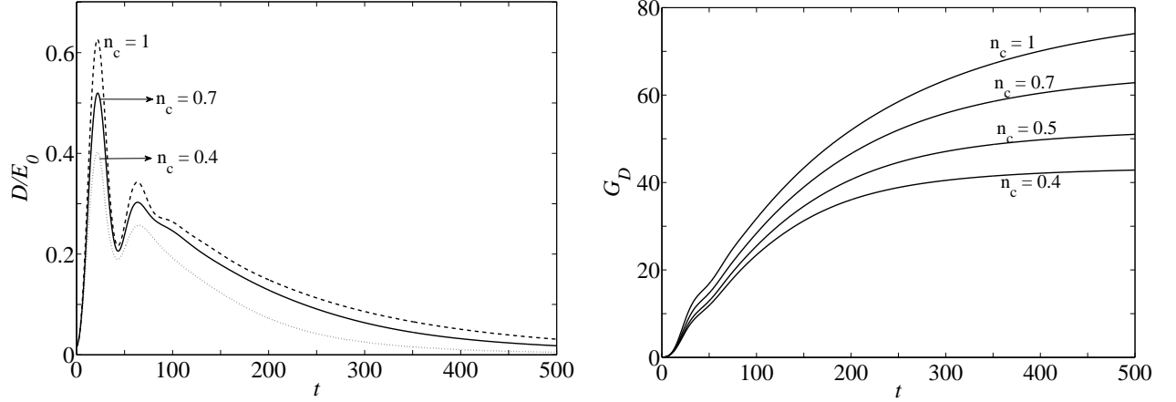
FIG. 18. Shear-thinning effects on the viscous dissipation.
