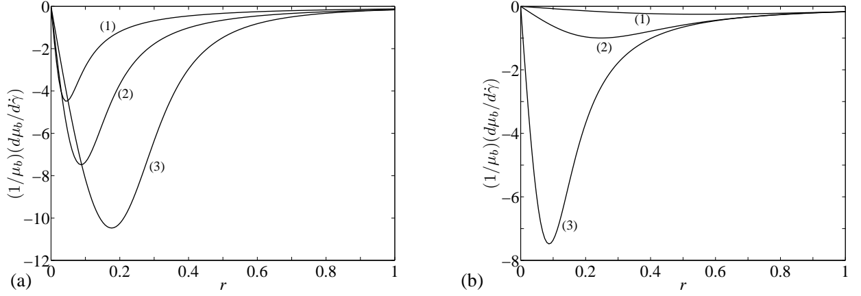
FIG. 3. Viscosity sensitivity. (a) \lambda = 30 and different values of the shear-thinning index: (1) n_c = 0.7 ; (2) n_c = 0.5 ; (3) n_c = 0.3 . (b) n_c = 0.5 and different values of the dimensionless constant time \lambda : (1) \lambda = 1 ; (2) \lambda = 4 and (3) \lambda = 30 .
