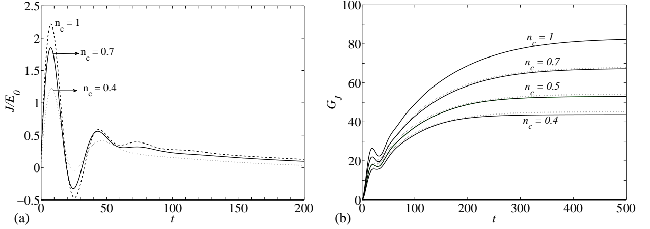
FIG. 14. Shear thinning effects on the production of the disturbance energy by the interaction of the Reynolds stress with the base flow. (a) Time evolution of the production rate J/E_0 . (b) Time evolution of \langle J \rangle_t / E_0 : (dotted line) purely stratified case, (continuous line) the viscosity perturbation is taken into account.
