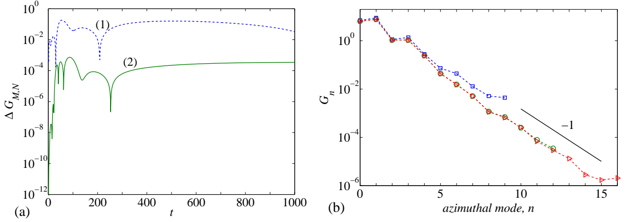
FIG. 7. Convergence test for a Carreau fluid n_c = 0.5 , \lambda = 30 at Re_w = 4000 . The initial perturbation is in the form of streamwise rolls with an energy \epsilon_0 = 10^{-2} . (a) Truncation error for two different spatial resolutions: (1) (M_1 = 6, N_1 = 9) and (2) (M_2 = 12, N_2 = 12) , with (M_h = 12, N_h = 16) . (b) Energy spectra over the azimuthal modes at t \approx 70 and for the three truncation levels tested: (\square) (M = 6, N = 9) ; (o) (M = 12, N = 12) and (\triangleright) (M = 12, N = 16) .
