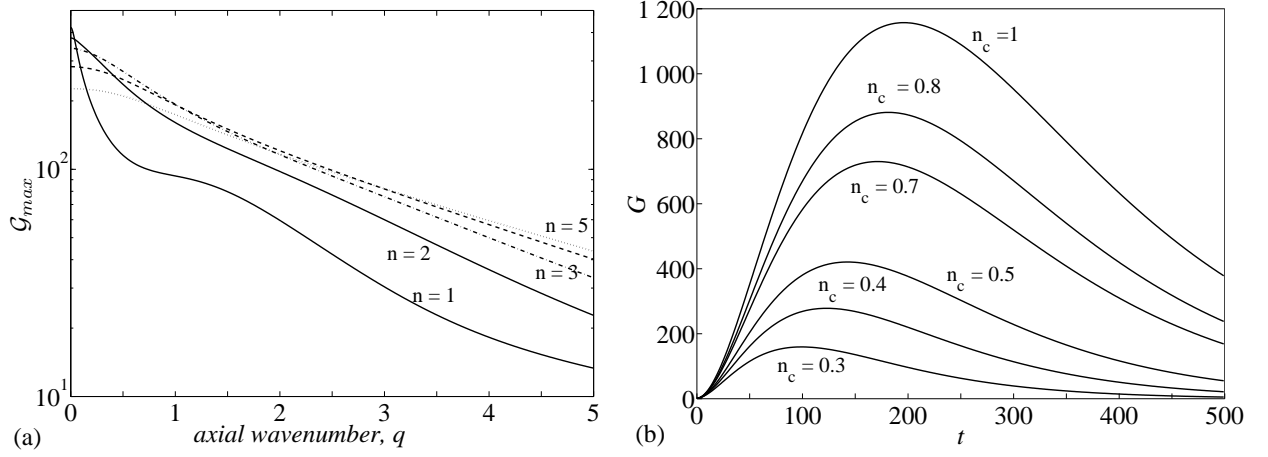
FIG. 4. (a) Maximum amplification of the disturbance kinetic energy as function of the axial wavenumber q for different azimuthal wavenumbers n at Re_w = 4000 , \lambda = 30 and n_c = 0.5 . (b) Gain of kinetic energy for the optimal perturbation at Re_w = 4000 , \lambda = 30 and different values of the shear-thinning index, n_c .
