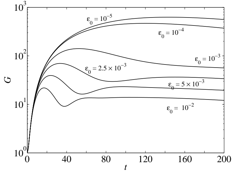
FIG. 6. Case of a Newtonian fluid. Energy amplification factor G(t) of a two-dimensional stream-wise perturbation at Re = 3000 and for different values of the initial energy \epsilon_0 . The results are obtained using M = 6 radial modes, N = 9 azimuthal modes and \Delta t = 0.01 .
