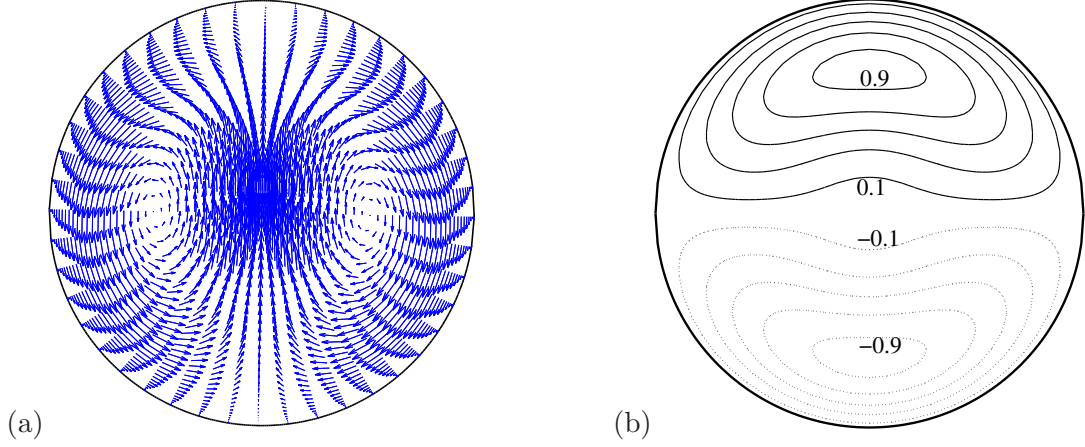
FIG. 5. (a) Optimal pattern of perturbation at t = 0 in the (r, \theta) section, for n_c = 0.5 , \lambda = 30 and Re_w = 4000 . The arrows represent the vectors ue_r + ve_\theta . (b) Optimal streaks at t = t^{opt} = 150 time units: Iso-values of the axial velocity component w . Continuous lines for positives values of w : 0.1 near the wall with a step of 0.2 until 0.9. Dashed lines for negative values of w : -0.1 near the wall then with a step of -0.2 until -0.9 .
