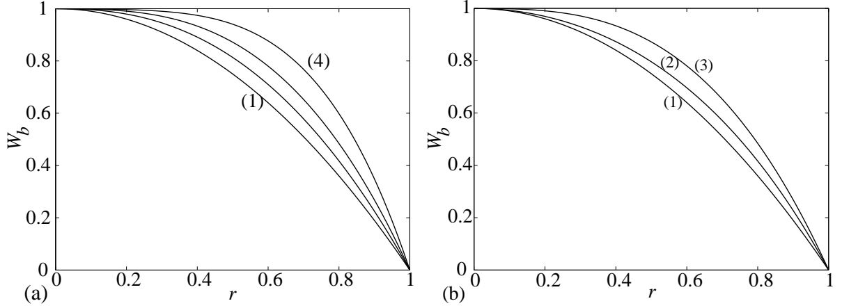
FIG. 1. Base velocity profiles. (a) \lambda = 30 and different values of the shear-thinning index (1) n_c = 1 Newtonian fluid; (2) n_c = 0.7 ; (3) n_c = 0.5 ; (4) n_c = 0.3 . (b) n_c = 0.5 and different values of the dimensionless constant time \lambda : (1) \lambda = 0 Newtonian fluid; (2) \lambda = 1 ; (3) \lambda = 30 .
