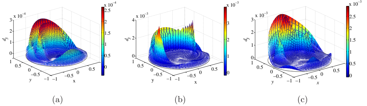
FIG. 16. Distribution in section r, \theta of the non-Newtonian Reynolds stress at three different times (a) t = 5 ; (b) t = 15 and (c) t = 150 . The computation is done with Re_w = 4000 and n_c = 0.5 .
