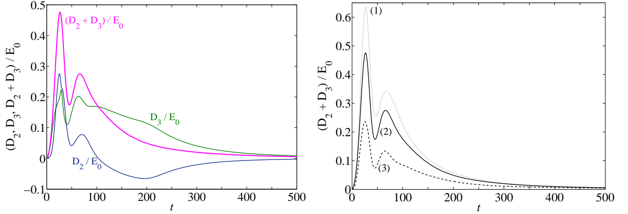
FIG. 15. (a) Time evolution of the additional terms D_2 and D_3 in the Reynolds-Orr equation arising from the viscosity perturbation at n_c = 0.5 and Re_w = 4000 . (b) Effect of the shear-thinning on (D_2 + D_3) / E_0 : (1) n_c = 0.4 , (2) n_c = 0.5 and (3) n_c = 0.7 .
