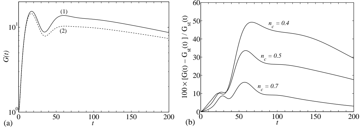
FIG. 9. (a) Energy amplification factor G(t) of a two-dimensional streamwise perturbation for a Carreau fluid with n_c = 0.5 at Re_w = 4000 : (1) the viscosity perturbation is taken into account, (2) the viscosity perturbation is not taken into account. (b) Relative variation between G(t) calculated when the viscosity perturbation is taken into account and that calculated without taking into account the viscosity perturbation. This latter case is called ‘purely stratified case’ and is indicated by the subscript st .
