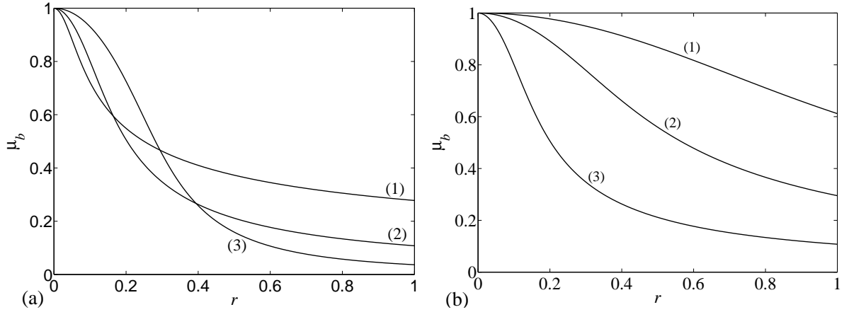
FIG. 2. Base viscosity profiles. (a) \lambda = 30 and different values of the shear-thinning index (1) n_c = 0.7 ; (2) n_c = 0.5 ; (3) n_c = 0.3 . (b) n_c = 0.5 and different values of the dimensionless constant time \lambda : (1) \lambda = 1 ; (2) \lambda = 4 ; (3) \lambda = 30 .
