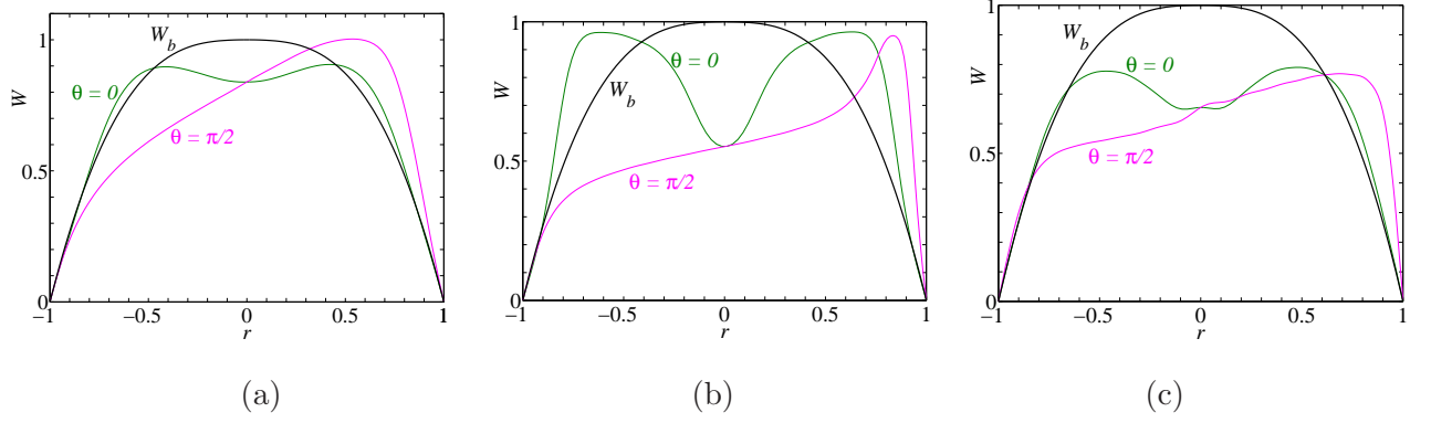
FIG. 12. Axial velocity profiles W_b(r) + w(r, \theta, t) of the perturbed flow at two azimuthal positions (horizontal \theta = 0 and vertical \theta = \pi/2 ). Case of Carreau fluid with n_c = 0.5 at Re_w = 4000 . The results are generated using M = 12 radial modes, N = 12 azimuthal modes and \Delta t = 0.01 . (a) t = 5 , (b) t = 15 and (c) t = 150 .
