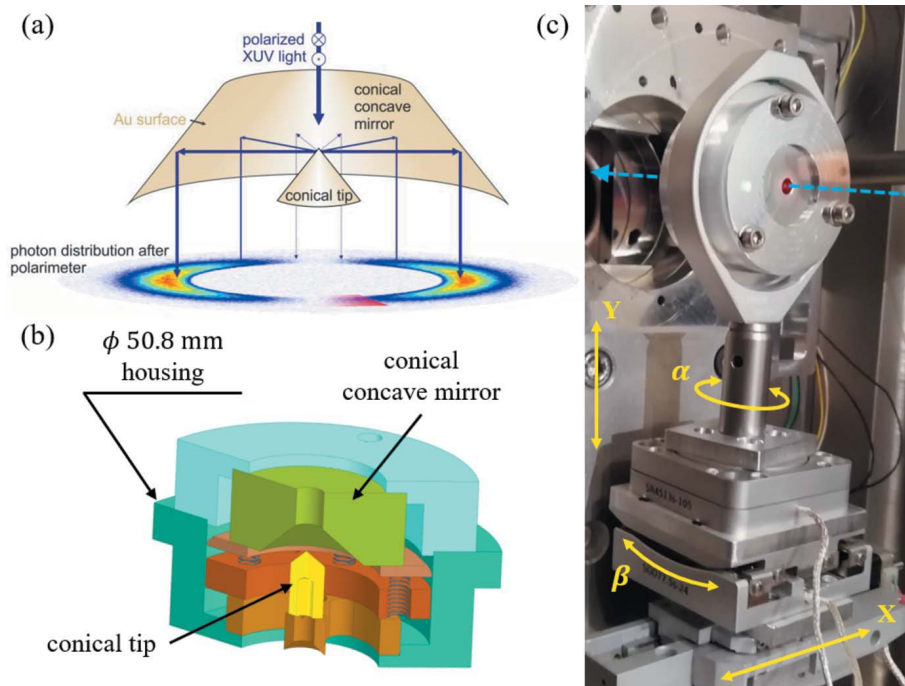
Figure 1 (a) Schematic view of the COMIX polarimeter. Due to the cylindrical symmetry, the transmitted intensity distribution depends on the polarization state of the incident beam. (b) Mechanical drawing of the COMIX polarimeter prototype, which can be mounted in standard optomechanical stages. (c) Four-axis motorized goniometer to precisely align the conical tip apex with respect to the XUV beam. The light blue dashed arrow shows the axis of the XUV beam, directed towards the CCD camera (not shown).
