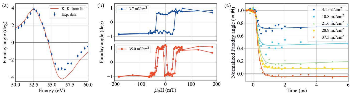
Figure 5 (a) Energy scan performed on the FeGd thin film around the Fe M_{2,3} -edge. The Faraday angle is measured between opposite saturation states, to be directly compared with the hysteresis loop amplitude. The red line shows data taken from von Korff Schmizing et al. (2020) and extracted from magnetic circular dichroism measurements via a Kramers-Kronig calculation. (b) Hysteresis loops measured at 53.9 eV for two different probing fluences. The experimental points have been obtained by fitting the polar profiles according to equation (3) and by removing from each loop its average value. (c) Delay scans measured at 52.8 eV for increasing pump fluences. The curve corresponding to the highest fluence shows magnetization inversion. The solid lines are fits performed according to equation (4).
