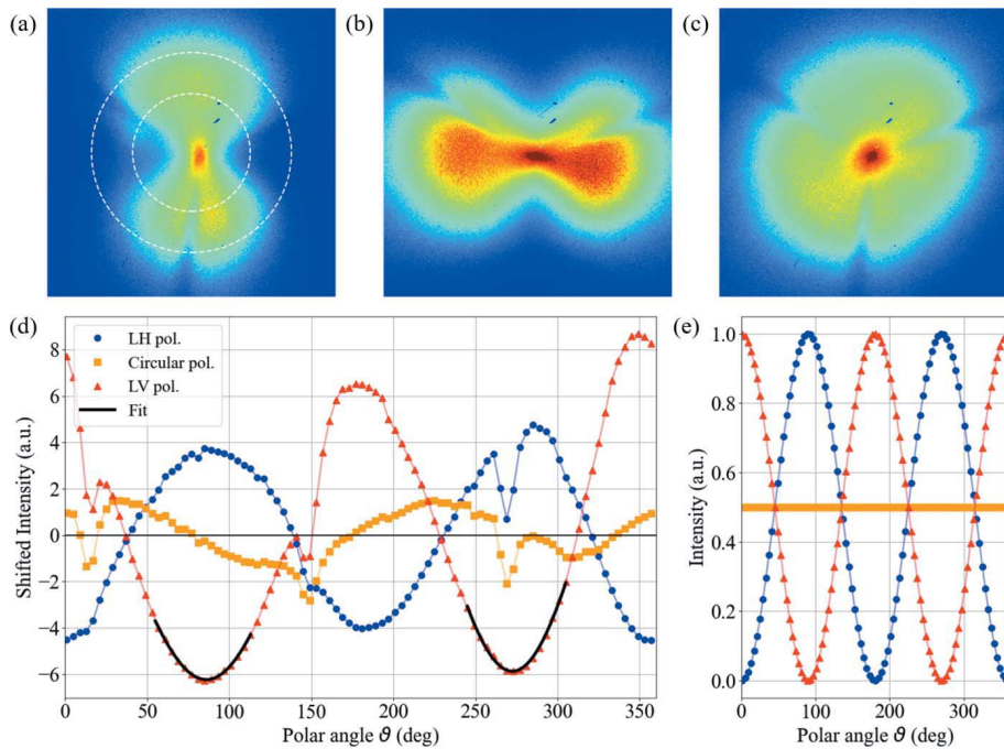
Figure 3 Intensity pattern recorded at 75 eV photon energy with nominally (a) LH, (b) LV and (c) circular polarization. The three images share the same colour bar and have been normalized to the incident beam intensity and to the exposure time. (d) Polar profiles obtained for images (a)–(c) within the region of interest depicted in panel (a). The glitch discontinuities at 30, 150 and 270° are due to the shadow of the mounting frame for the inner conical mirror. (e) Calculated polar profiles for ideal polarization states obtained from equation (2), to be compared with panel (d).
