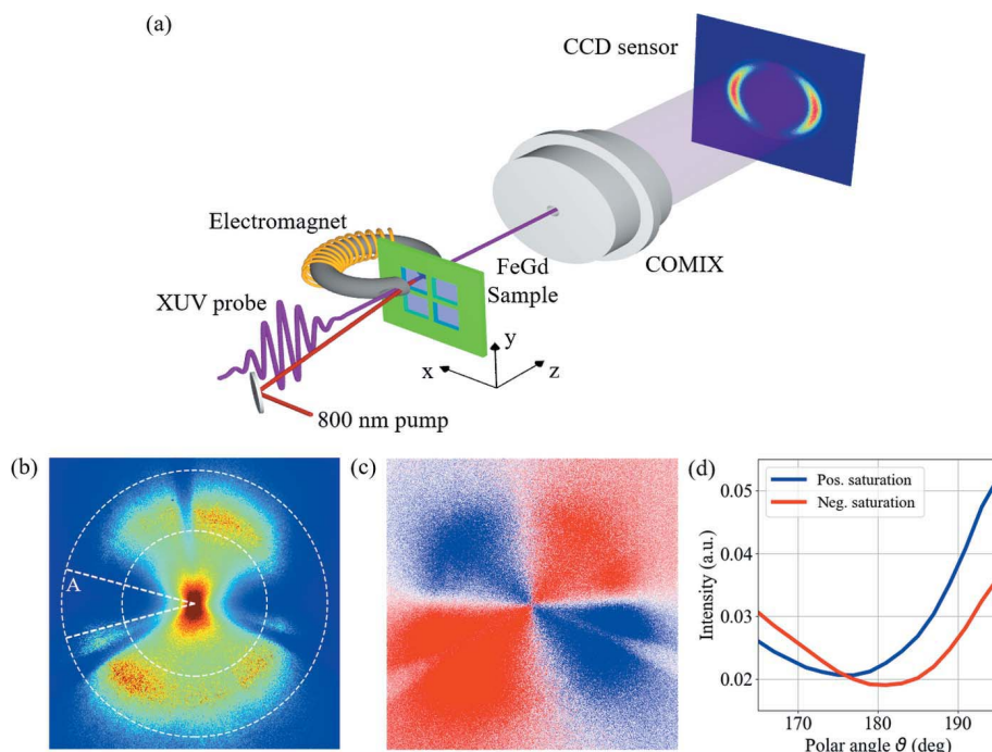
Figure 4 (a) Sketch of the experimental setup for time-resolved pump–probe measurements. (b) Intensity pattern recorded with LH polarized light tuned to 52.8 eV when the FeGd thin film was saturated along the z axis (positive saturation). (c) Difference signal between panel (b) and the corresponding image obtained saturating the sample in the opposite direction (negative saturation). By doing so, the common background can be removed, and the relative changes are highlighted. (d) Polar profiles obtained in a ±15° range around the intensity minimum labelled by A for panel (b) and for the corresponding image obtained at negative saturation. After fitting, a relative Faraday rotation of (4.6 ± 0.4)° has been evaluated.
