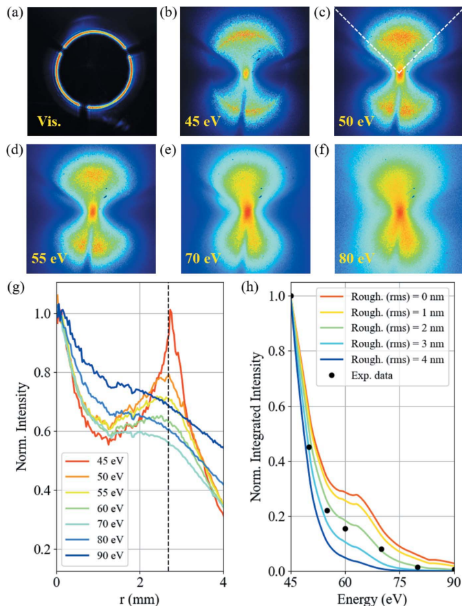
Figure 2 (a) Recorded intensity pattern obtained with unpolarized visible light. A circular ring-like structure is clearly visible. (b)–(f) Recorded intensity pattern obtained with LH polarized light of increasing photon energy, as stated in the labels. The colour bar limits are different for each panel, and they have been chosen to better highlight the features of interest. (g) Radial profiles extracted from the region contained between the two white dashed lines in (c). All the profiles are normalized to the intensity at the centre of the image ( r = 0 ). The vertical black dashed line highlights the average radius of the circular structure in (a). For increasing energy, the amplitude of the peak corresponding to the ring-like feature decreases, while its width is enhanced. (h) Normalized integrated intensity as a function of the photon energy. The black dots represent the experimental data, while the continuous colour lines show the predicted energy dependence of the COMIX transmittance for mirror roughnesses in the 0–4 nm (r.m.s.) range.
