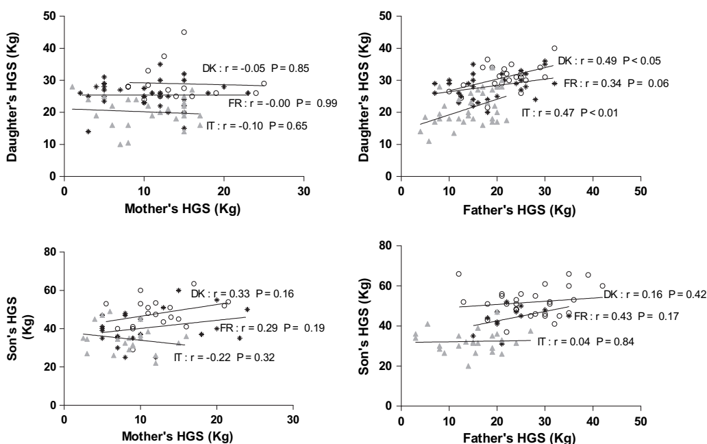
Figure 1. Correlations between parental and offspring handgrip strength (HGS) in each European region. Open circle, Southern Denmark (DK); asterisk, Languedoc-Roussillon, France (FR); shadowed triangle, Calabria, Italy (IT). Note: r = Pearson correlation coefficient.
