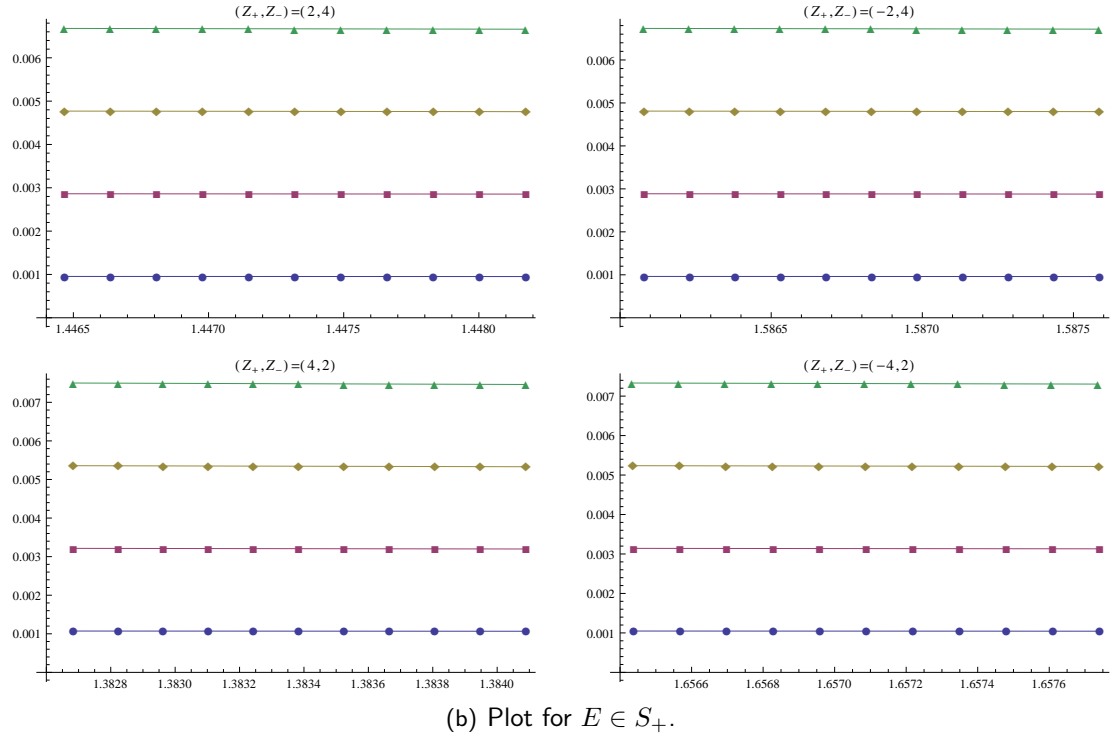
Figure 7.4: Renormalised resonances E/\ell(\mathfrak{R}(E)) with parameters h = 0.001 , C = 9 and m = 9000, \dots, 9010 .
