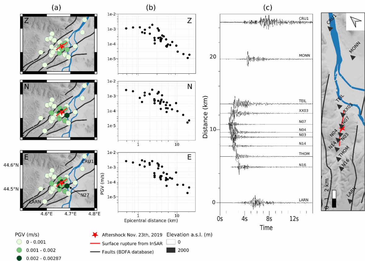
Figure 10. (a) Spatial distribution of Peak Ground Velocity (PGV) recorded by the three components (Z, N, E) of ground motion after the November 23, 2019, Ml 2 aftershock (SISMALP location). Seismograms are band-pass filtered between 0.1 and 20 Hz. N27 station location is indicated by the arrow. (b) PGV as a function of epicentral distance. (c) Velocities recorded by the NS component of stations lying along a SW-NE section (from LARN to CRU1 stations, see (a)). Velocities are band-pass filtered between 0.5 and 10 Hz and, for the sake of clarity, each seismogram is normalized by its peak ground value.
